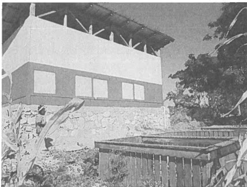
Fig. 12. Human waste composting latrines: designed by Give Love and maintained by local people, these latrines address a sanitation need, and the harvested compost is used in community gardens or sold.
