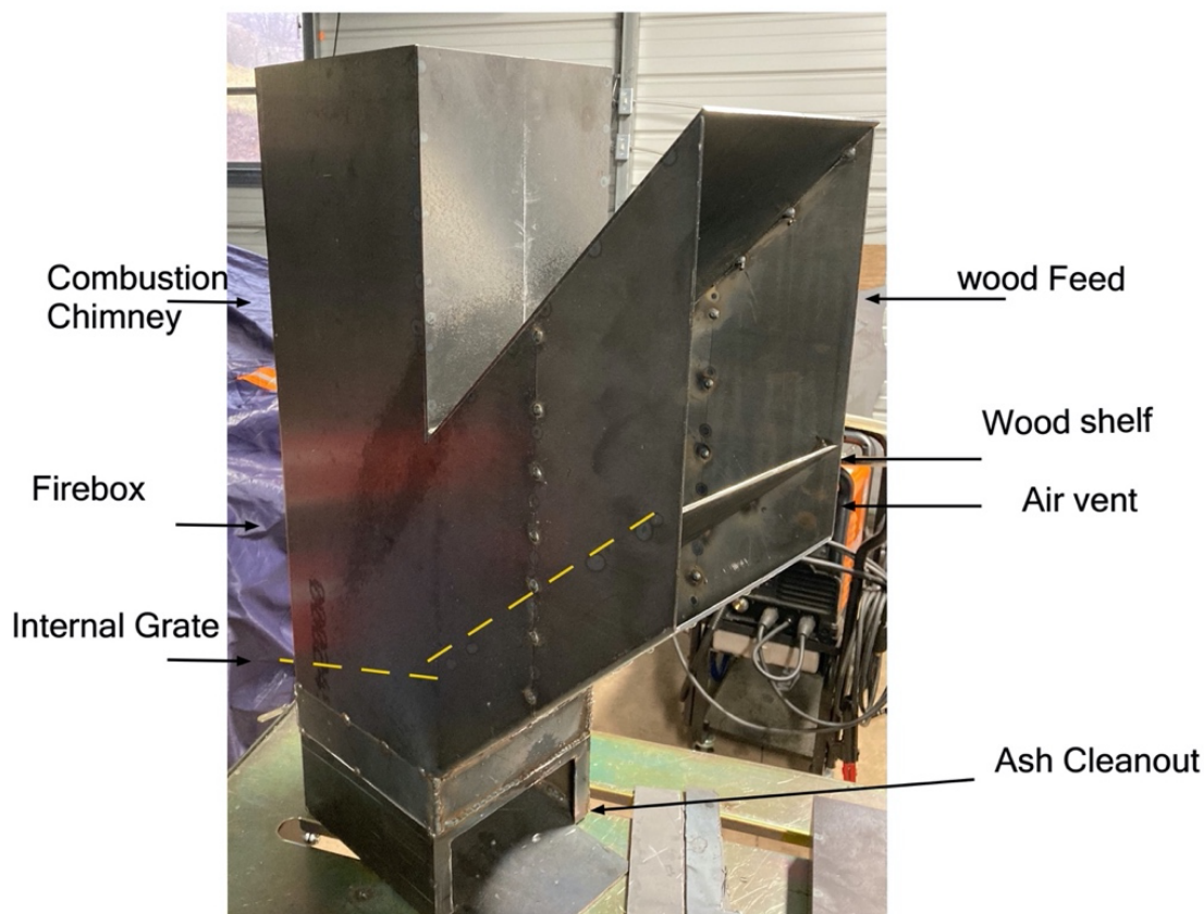
Figure 1 – Internal Components of Rocket Sap Evaporator
