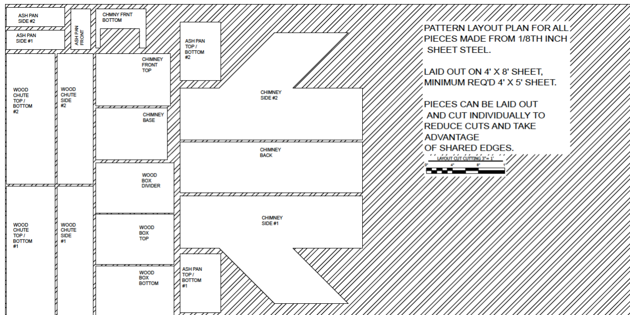
Figure 1: Pattern Layout for 1/8th Inch Sheet Steel for most compact use of steel
