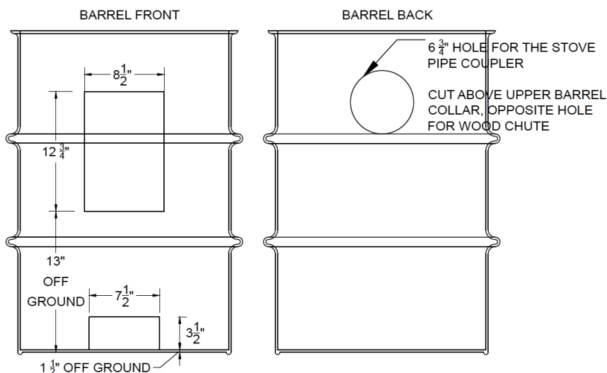
Figure 6: Barrel cut-out dimensions
