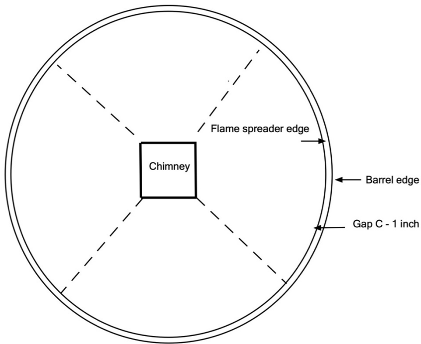
Figure 3 – Flame spreader
